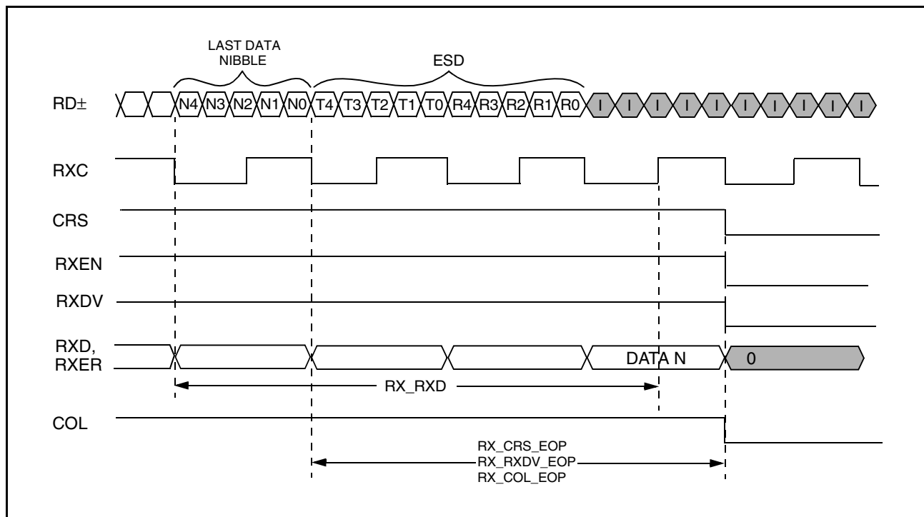
Figure 8: MII Receive End of Packet Timing (100BASE-TX)
